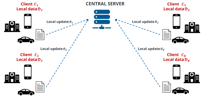
Fig. 3. FL framework overview.
