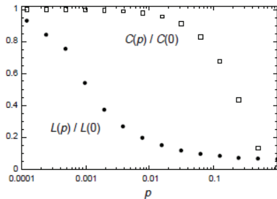
Figure 4.3: The change of the clustering coefficient and the diameter as p increases from 0 to 1. From [11].
