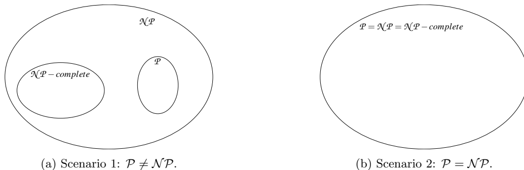
Figure 15: Relationship between the \mathcal{NP} and the \mathcal{P} problem classes. One of the two possible scenarios holds but we do not know which one.
